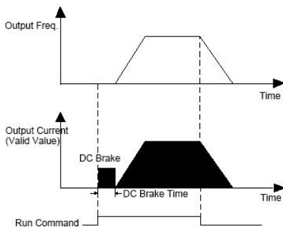
Figure F6-2 start DC brake
