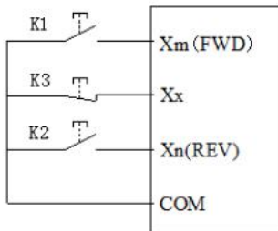
Fig. F4-4 3-wire Control Mode 1
