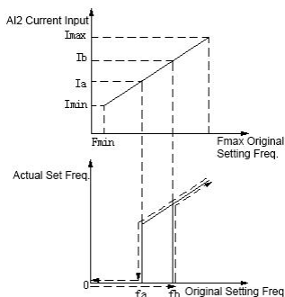
Fig. F4-6 zero-frequency function schematic diagram
