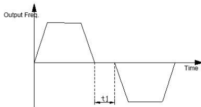
Fig. F1-7 FWD/REV run dead band time
