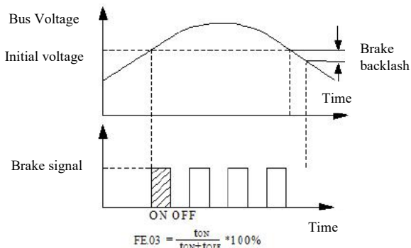
Fig. FE-1 Dynamic Braking
